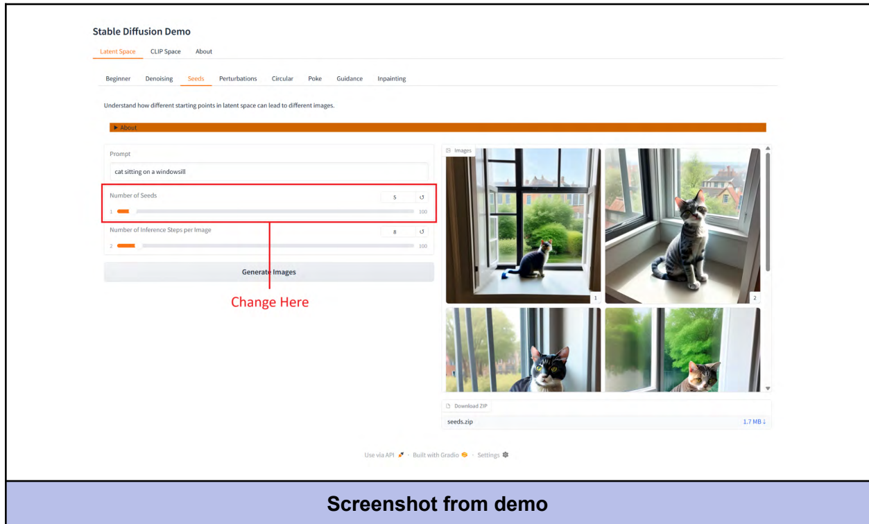
Figure 8 - Change the number of seeds with the Number of Seeds slider.
