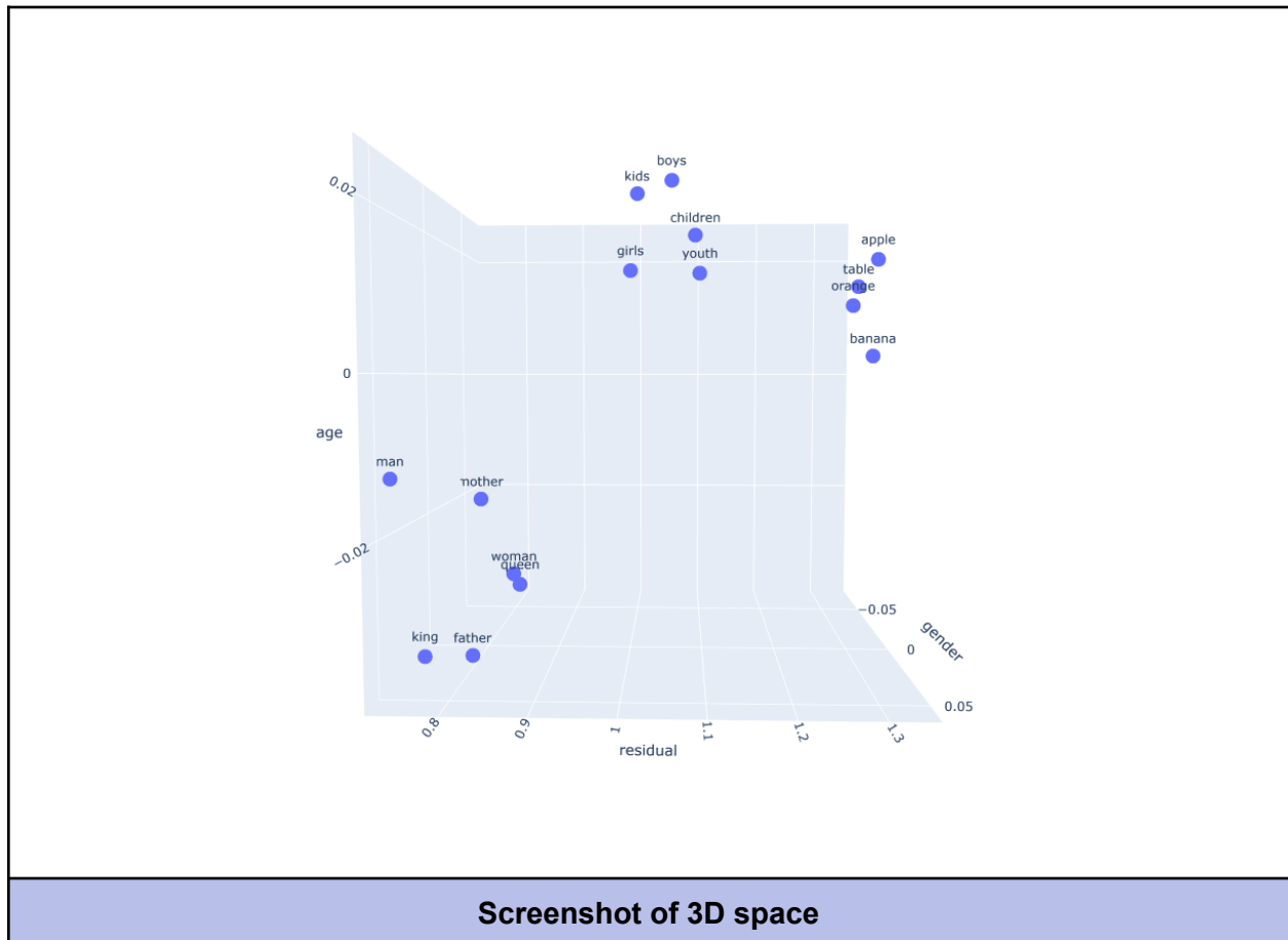
Figure 35 - Organization of multiple words in CLIP space.
